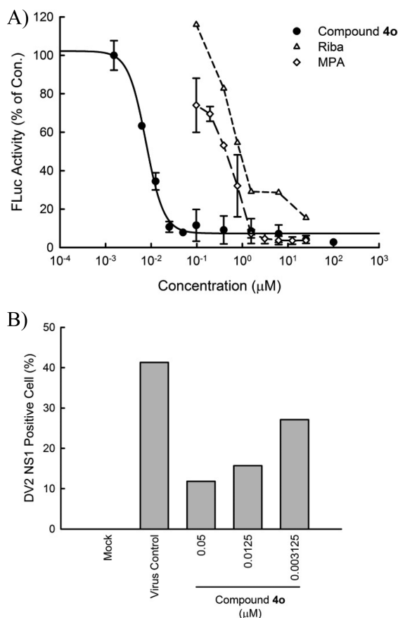
Figure 2. (A) Antiviral activity of 4o and reference compounds in BHK-DV2-replicon cell line. (B) Validation of 4o antiviral activity using an infectious DENV-2 virus in BHK cells.
