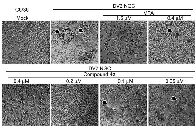
Figure 3. Antiviral activity of 4o in C6/36 cell line infected by DENV-2 virus.
