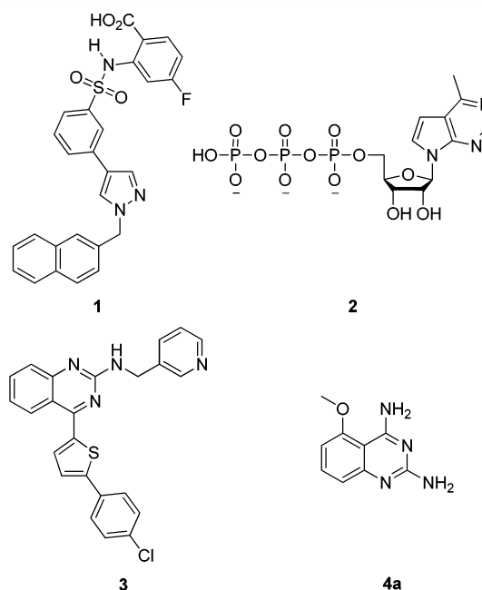
Figure 1. Recently uncovered DENV inhibitors and 4a .
